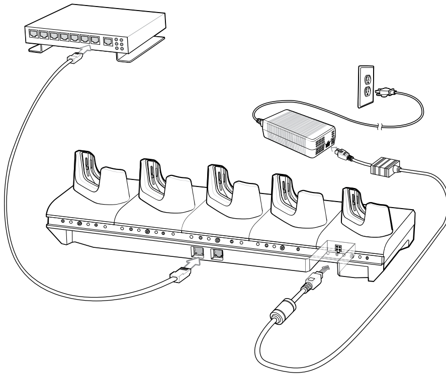
Figure 46 5-Slot Ethernet Cradle Setup
