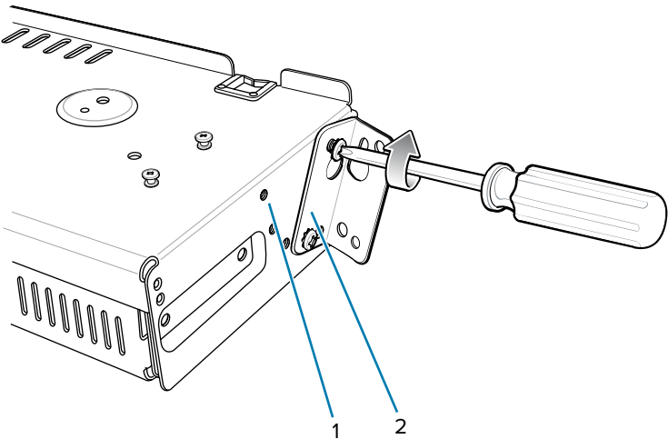
Figure 51 Flange 25° Position (4-Slot Battery Chargers)
