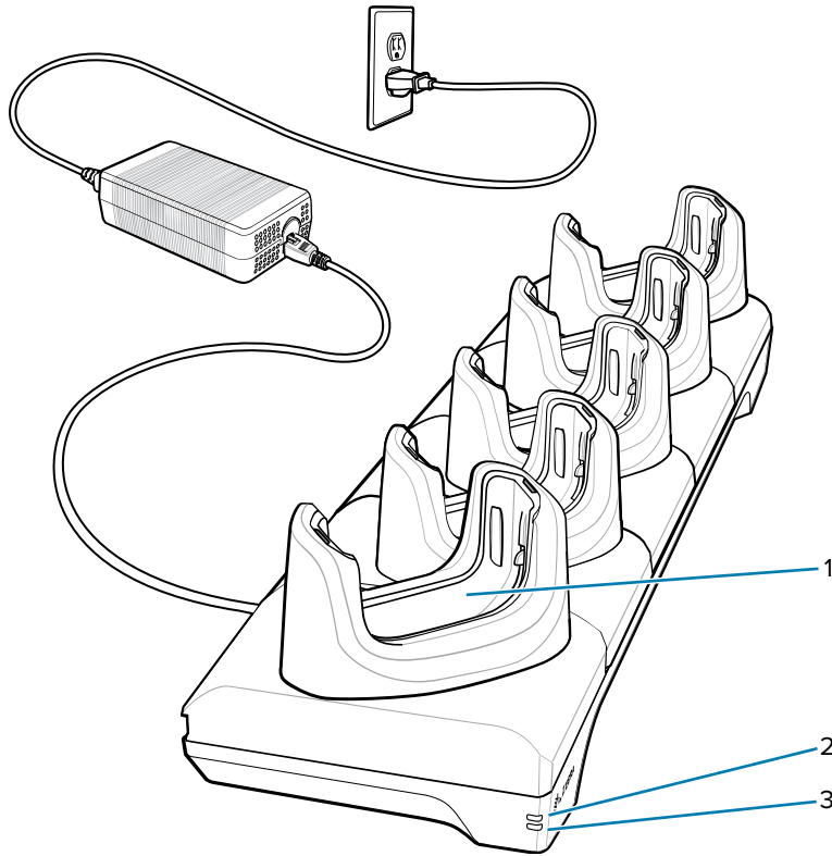
Figure 45 5-Slot Ethernet Cradle
