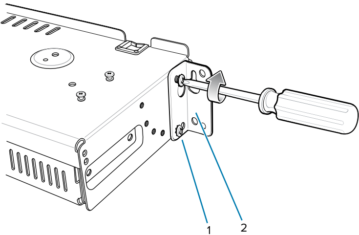
Figure 50 Flange Horizontal Position (5-Slot Cradles)
