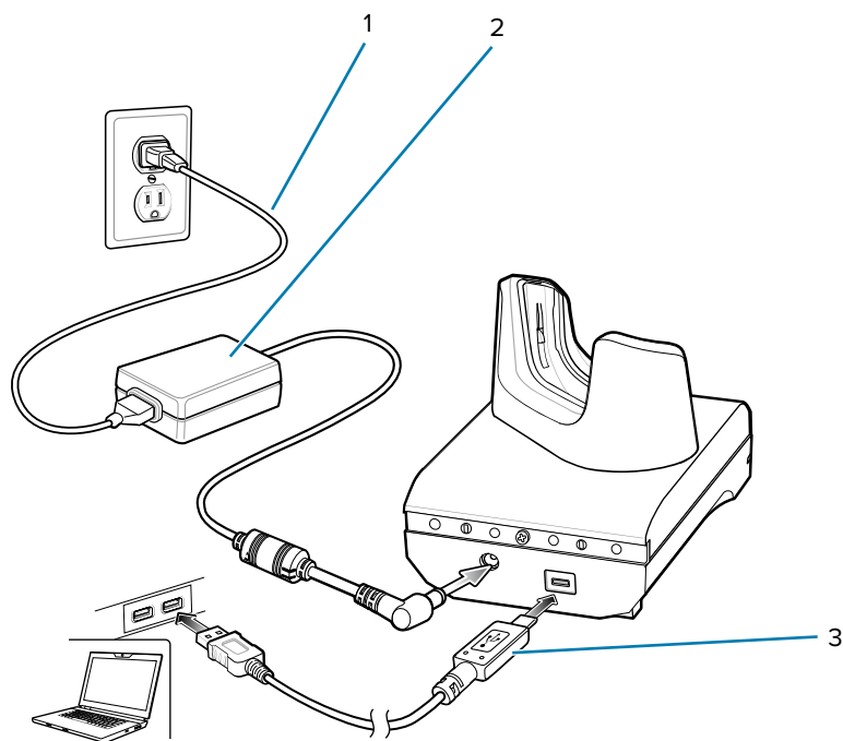
Figure 34 1-Slot USB Charge Cradle Setup
