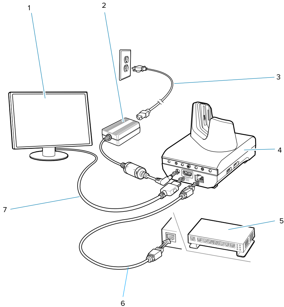
Figure 36 Workstation Cradle Setup
