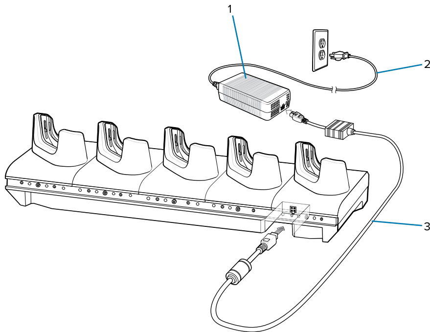
Figure 43 5-Slot Charge Only Cradle Setup
