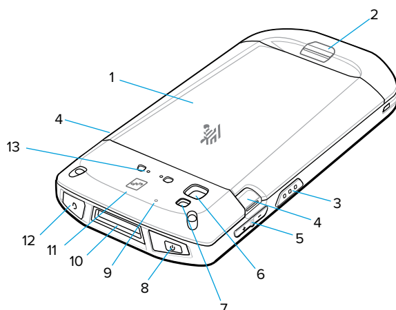
Figure 2 TC52x Rear View
